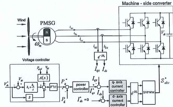
Fig. 2: Control block diagram of the machine-side converter.
