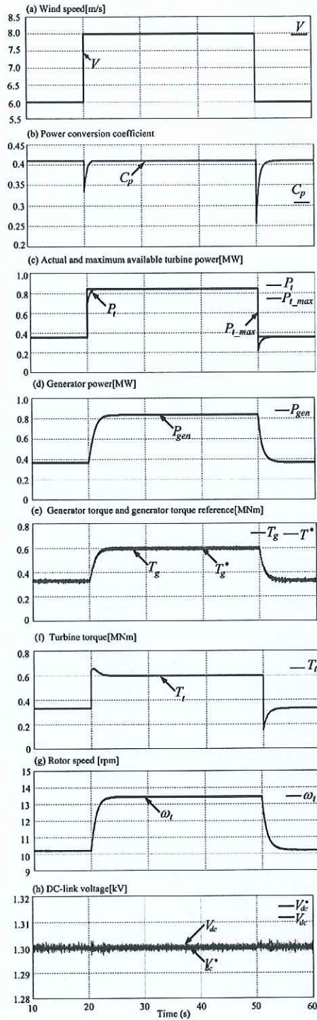
Fig. 8: Responses of optimal torque control in step-wise wind speed variation: (a) wind speed, (b) power conversion coefficient, (c) actual and maximum available turbine power, (d) generator power, (e) generator torque and generator torque reference, (f) turbine torque, (g) rotor speed, (h) DC-link voltage.
