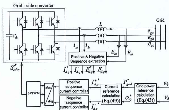
Fig. 7: Control block diagram of the grid-side converter.
